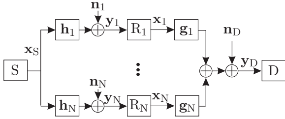
Fig. 1. Block diagram of a relay network with N parallel relays
