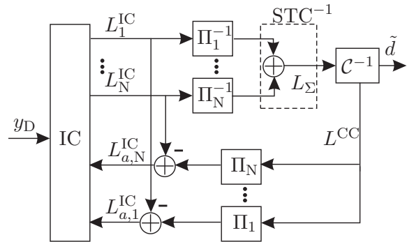
Fig. 2. Block diagram of the IDM-STC detector
