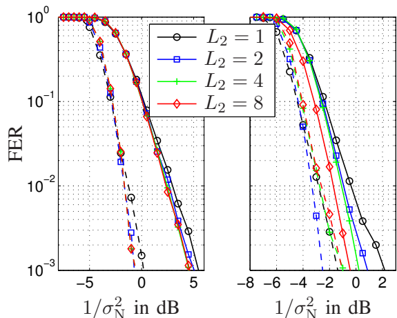
Fig. 6. Frame Error Rate in a network with 4 relays with IDM-STC (- -) and OFDM-CDD (-), 1st hop AWGN and second hop Rayleigh fading channels of different length, convolutional code with L_c = 3 (left) and L_c = 7 (right)
