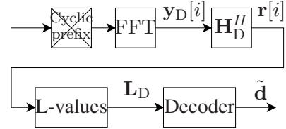
Fig. 4. Block diagram of the destination for OFDM-CDD
