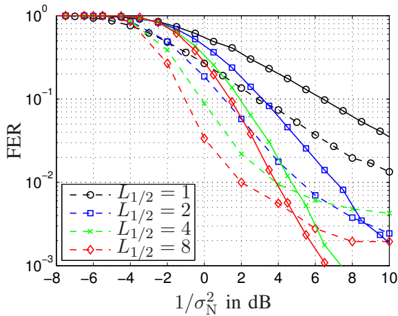
Fig. 7. Frame Error Rate in a network with 4 relays with IDM-STC (- -) and OFDM-CDD (-), both hops Rayleigh fading of different length, convolutional code with L_c = 3
