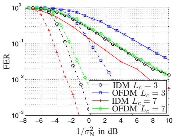
Fig. 5. Frame Error Rate in a network with 4 relays, 1st hop AWGN (- -) or Rayleigh fading (-)
