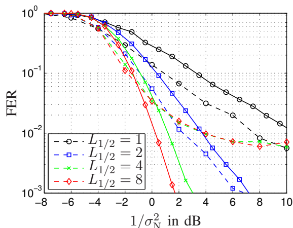
Fig. 8. Frame Error Rate in a network with 4 relays with IDM-STC (- -) and OFDM-CDD (-), both hops Rayleigh fading of different length, convolutional code with L_c = 7
